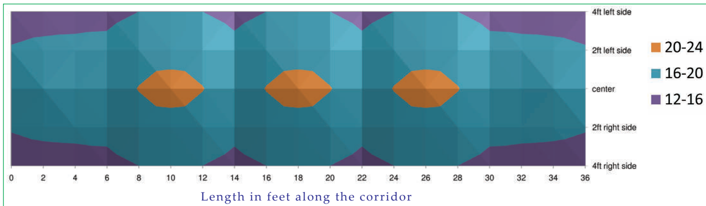
LUX Distribution Pattern
